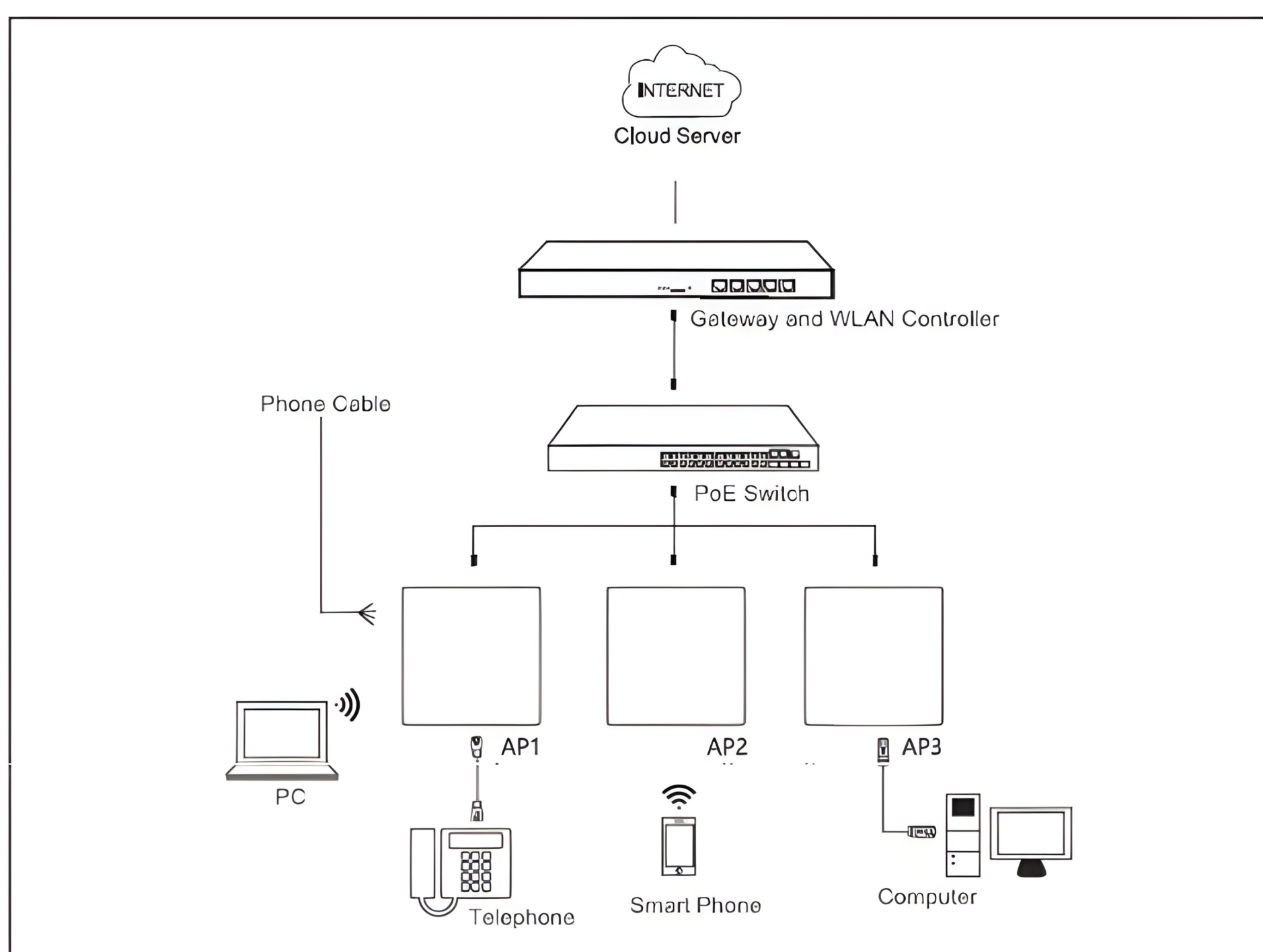
Figure 1. Rizonn access points with on-premise controller.
